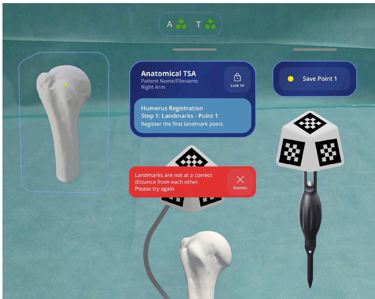
Figure 32: Signature Vision Application Humerus Registration Step - Landmark Registration Failed
